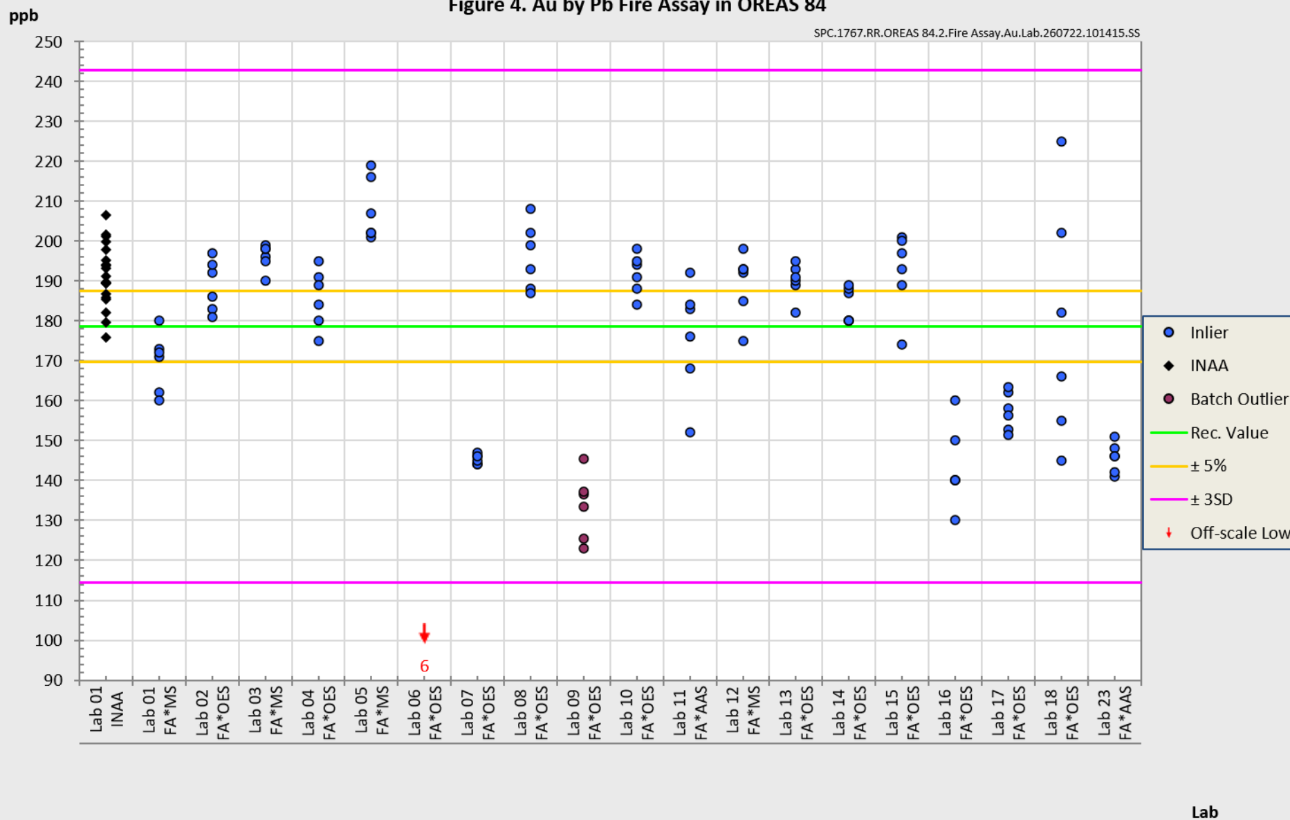
Figure 4. Au by Pb Fire Assay in OREAS 84
