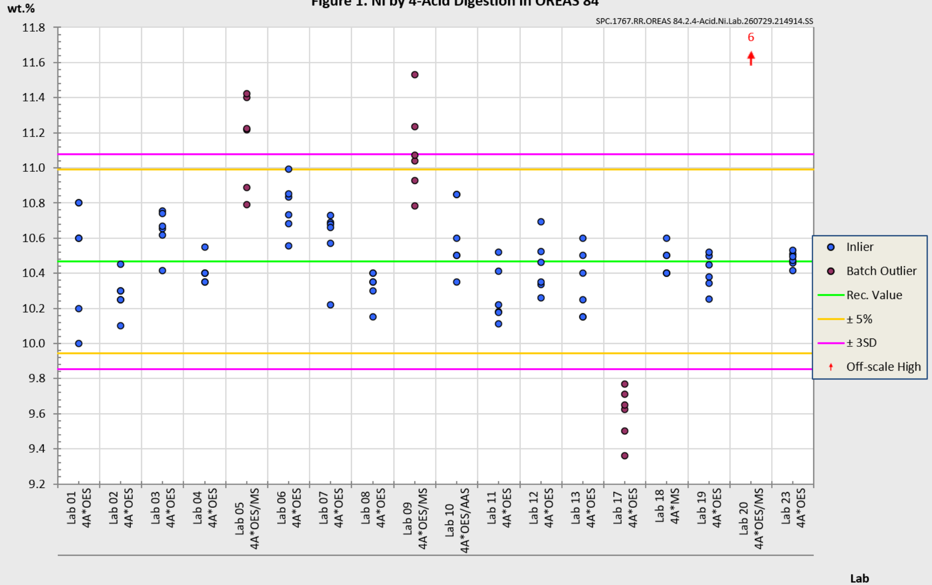
Figure 1. Ni by 4-Acid Digestion in OREAS 84
