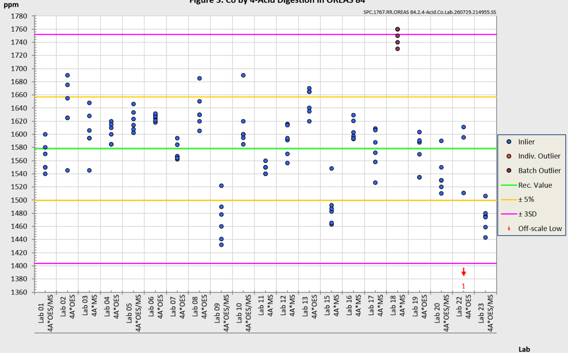
Figure 3. Co by 4-Acid Digestion in OREAS 84
